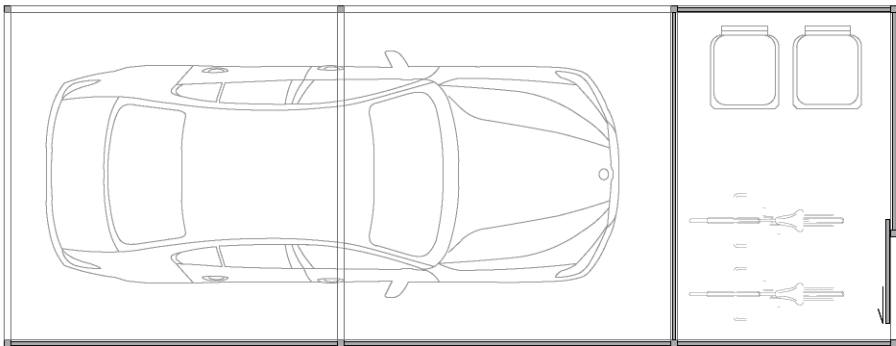
CARPORT WITH RECYCLABLES AND BICYCLE ENCLOSURE Carport wall panels: Perforated sheet in RAL, surface-mounted: Natural larch wooden battens, roof panel: Trapezoidal sheet metal
